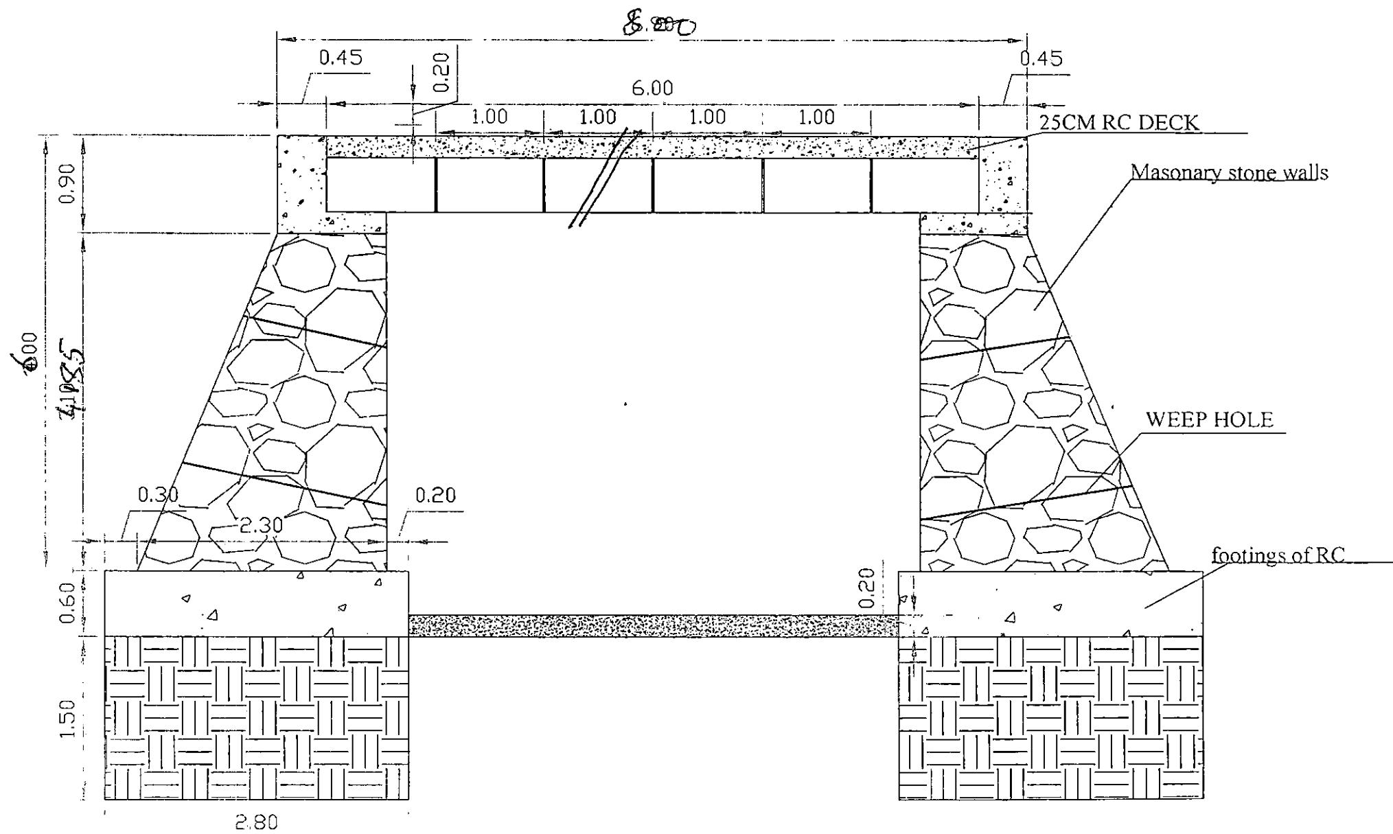
LONGITUDINAL SECTION. OF THE BRIDGE
