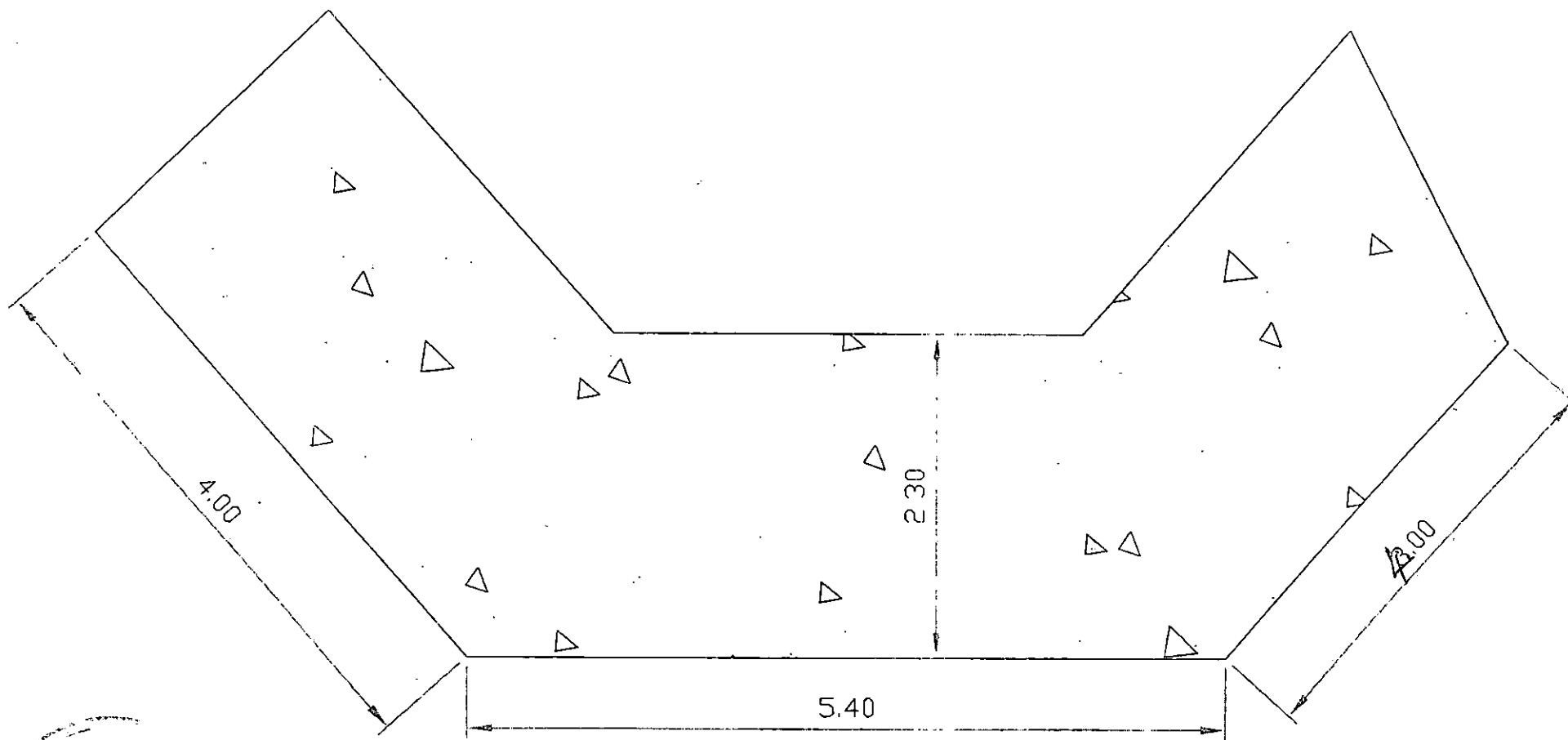
DETAIL FOOTING
