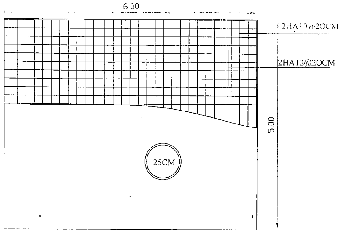
REINFORCEMENT PLAN
